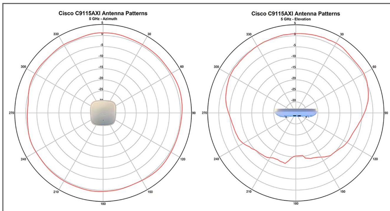
Figure 1. Antenna radiation pattern
