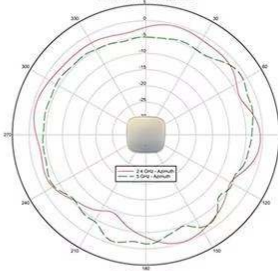
Cisco C9120AXI Antenna Patterns Azimuth - Dual Band AUX Antenna
