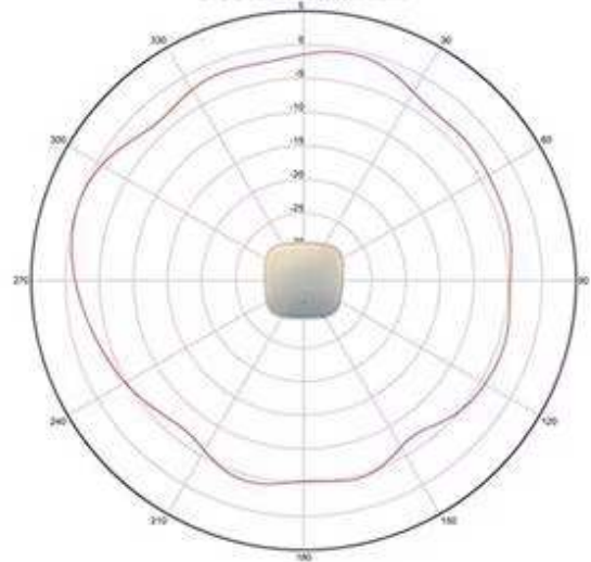
Cisco C9120AXI Antenna Patterns 2.4 GHz - Azimuth - Bluetooth Antenna
