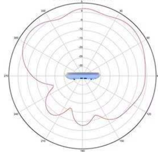
Cisco C9120AXI Antenna Patterns 2.4 GHz - Elevation - Bluetooth Antenna
