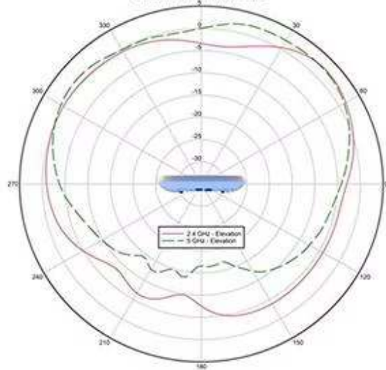
Cisco C9120AXI Antenna Patterns Elevation - Dual Band AUX Antenna
