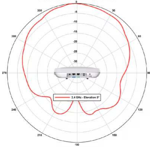
Catalyst 9166D1 Series Wi-Fi 6E Access Points 2.4 GHz - Elevation 0° - Client Serving - Normalized
