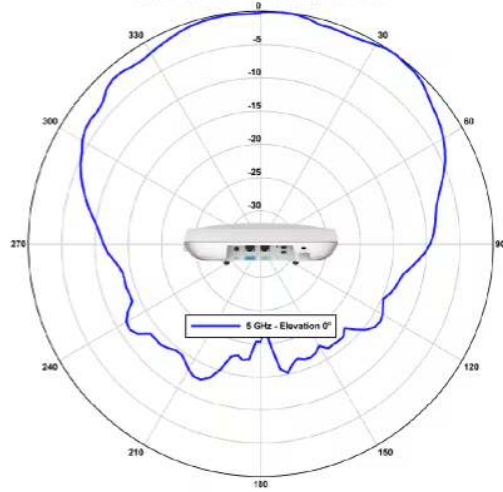
Catalyst 9166D1 Series Wi-Fi 6E Access Points 5 GHz - Elevation 0° - Client Serving - Normalized
